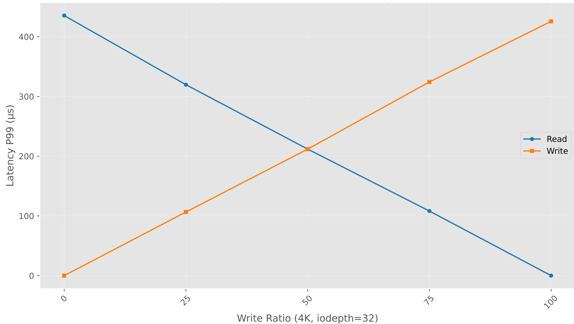
Latency P99 vs Write Ratio (4K, iodepth=32)
